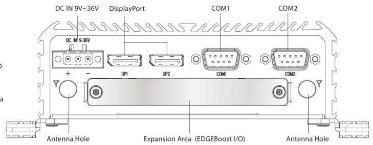
Rear Panel
