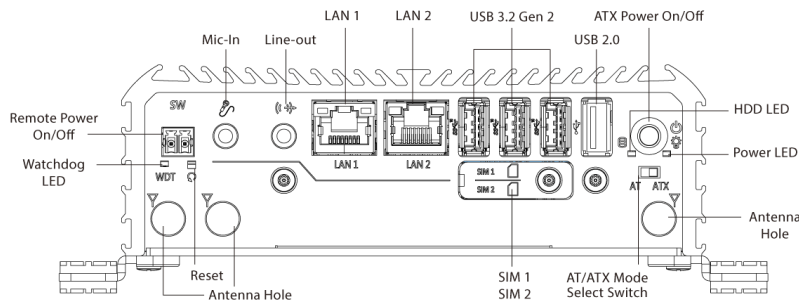
Front Panel
